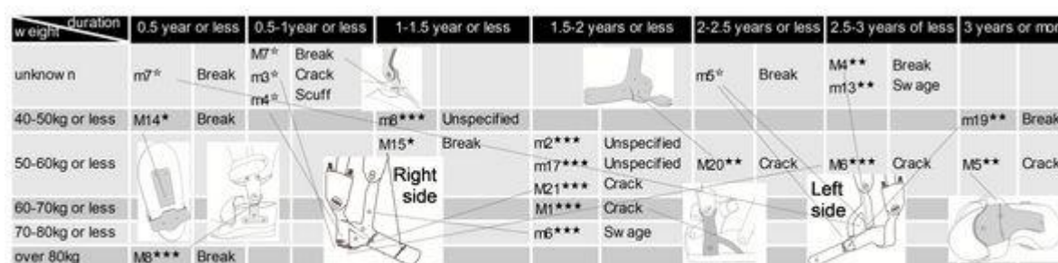
Figure 1. Damages of stirrup and/or foot plate with double-upright AFO (20 cases)
