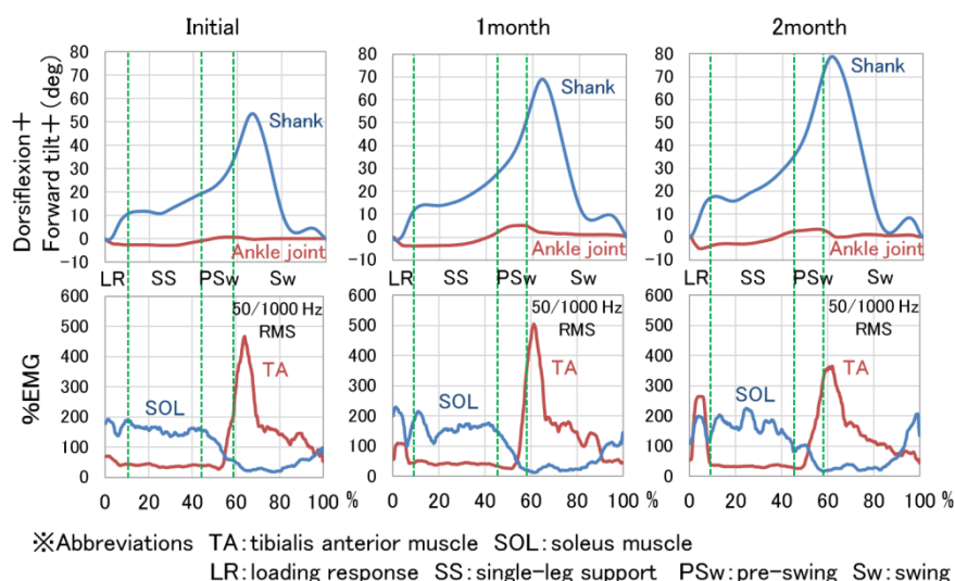
Figure 1. Typical examples of angle and EMG waveform
