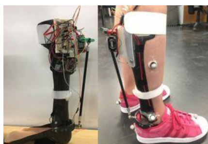
Figure 1. Developed AAFO.
