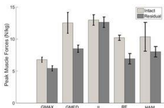
Figure 1. Peak of hip muscle forces in stance. Symbols are GMAX: gluteus maximus; GMED: gluteus medius; IL: iliopsoas; RF: rectus femoris; HAM: hamstrings
