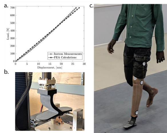
Figure 1: (a) Instron-measured and FEA calculated vertical displacements under loads applied at a horizontal distance of 13 cm from the ankle (b) Photograph of the experimental setup (c) Indian amputee walking on level ground with the foot prototype.
