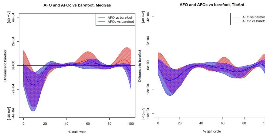
Figure1. Difference plots with 95% confidence intervals for medial gastrocnemius(left) and tibialis anterior(right). The plots depict the difference from barefoot to orthotic conditions with AFO in red and AFOc in blue. Significant change is detected where outer plot limits clear the x-axis.
